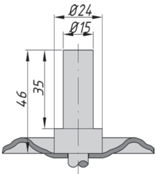
dotyczy obudów do kół / for housings with wheels \varnothing 80 \div \varnothing 125M
