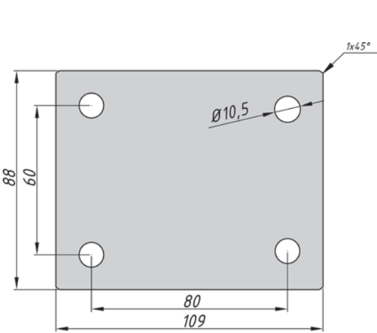
dotyczy obudów do kół / for housings with wheels \varnothing 80 + \varnothing 125M
