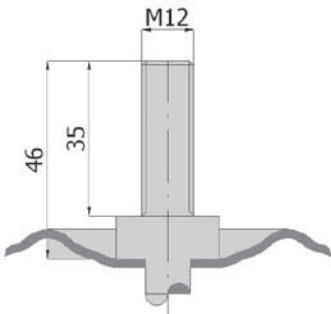
dotyczy obudów do kół / for housings with wheels \varnothing 80 \div \varnothing 100
