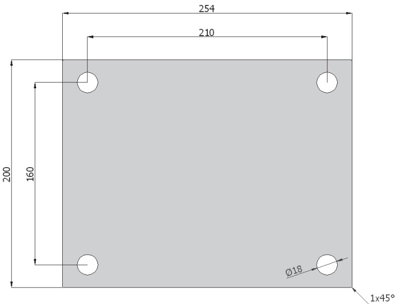
dotyczy obudów tandem do kół / for tandem housings with wheels \varnothing 350
