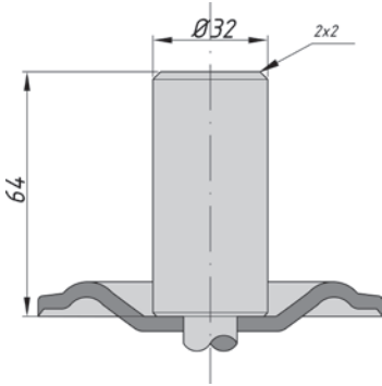
dotyczy obudów do kół / for housings with wheels \varnothing 125 \div \varnothing 200
