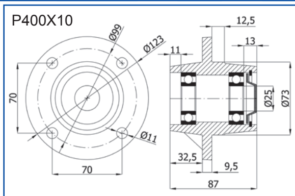
P400X10 - piasta koła (400/10) / wheel hub (400/10)
